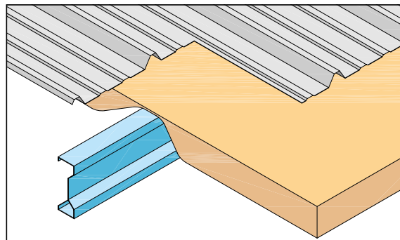
ATLAS-Clad-Dach ACR 40/0i.
